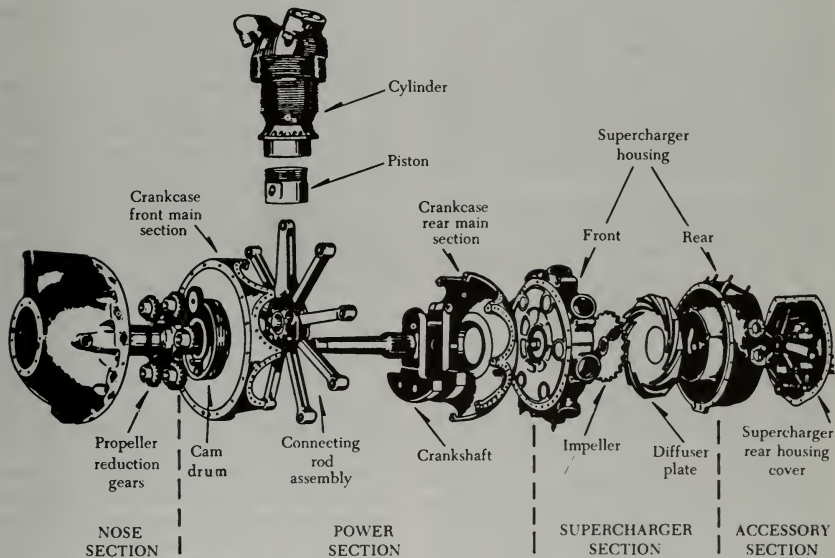
FIGURE 1-6. Engine sections.
